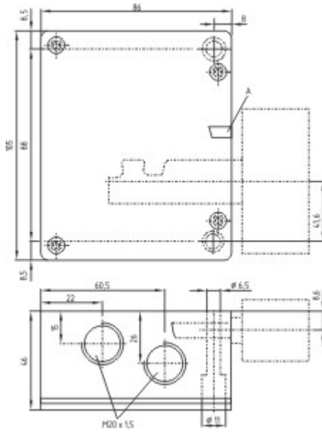
Dimensional drawing (basic component)
